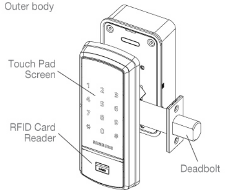
Outer body
